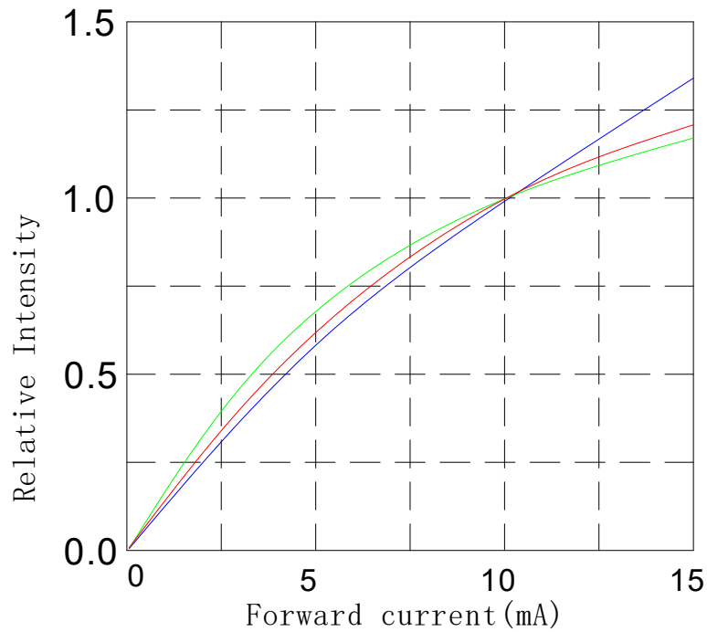
Figure 3. Relative Intensity vs. forward current for Lumileds 5050 RGB R at T=25^\circ\text{C}
