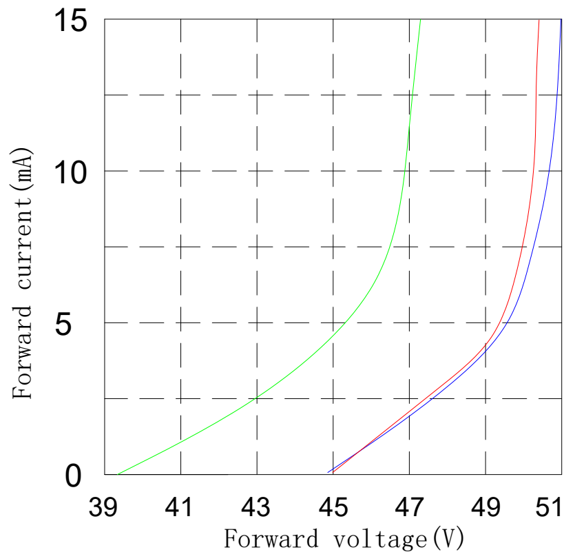
Figure 4. Typical forward current vs. forward voltage for Lumileds 5050 RGB R at T=25^\circ\text{C} .
