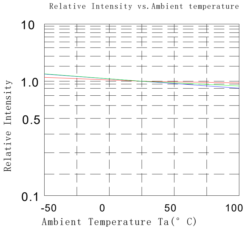
Figure 2 . Relative Intensity vs.Ambient temperature for Lumileds 5050 RGB R at 30mA .
